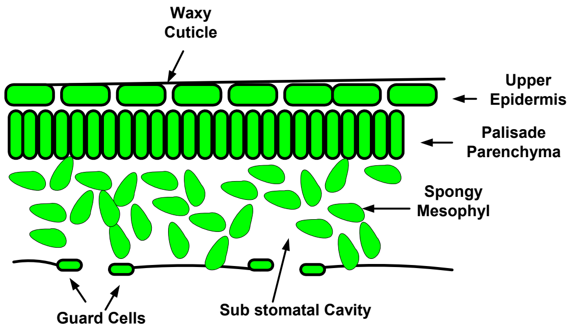
Figure 16 Cross section of a leaf with the \text{C}_3 photosynthetic pathway
