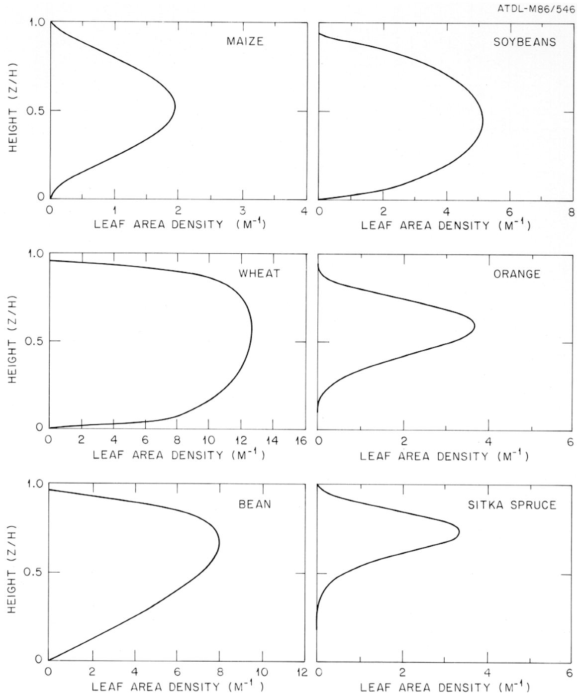
Figure 23 Examples of leaf area index profiles for crops and forests. Meyers and Paw U, 1986
