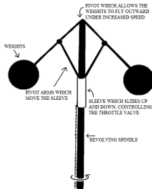
James Watt's Governor
