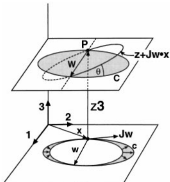
Figure 12 The graph of g near c_i asymptotically approximated by the plane z = z_i + \mathbf{J}\mathbf{w}_i \cdot \mathbf{x} , where \mathbf{w}_i is the rotation vector.
