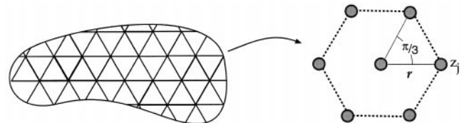
FIGURE 3 Configuration of seven proteins, with one at the origin and six at the vertices of a regular hexagon.
