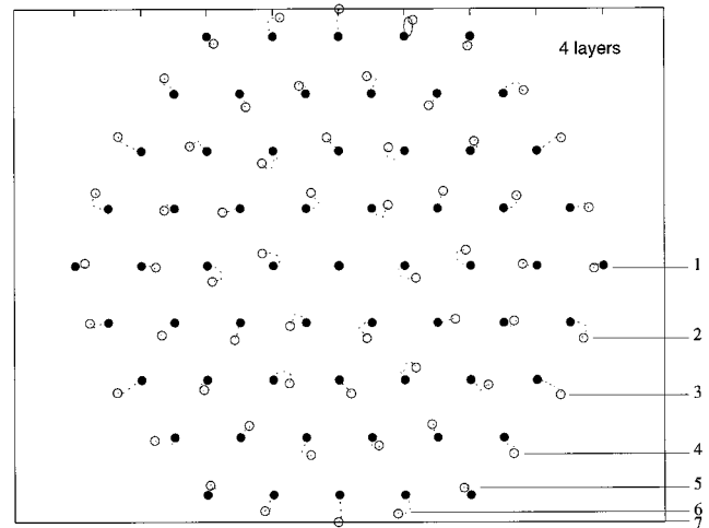
FIGURE 4 N = 61 protein lattice simulation. The initial positions are represented by black dots, and the positions of the proteins at the end of the run are represented by open circles. The final and initial values of |\eta_i| at seven selected boundary proteins (labeled from 1 to 7) are as follows: (1) 0.0008 (2.3051); (2) 0.0008 (0.3221); (3) 0.0008 (0.1111); (4) 0.0008 (0.3221); (5) 0.0018 (2.3051); (6) 0.0008 (0.3221); (7) 0.0008 (0.1111).
