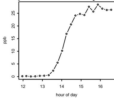
pinonaldehyde
