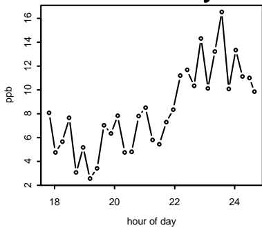
cycloheptene
