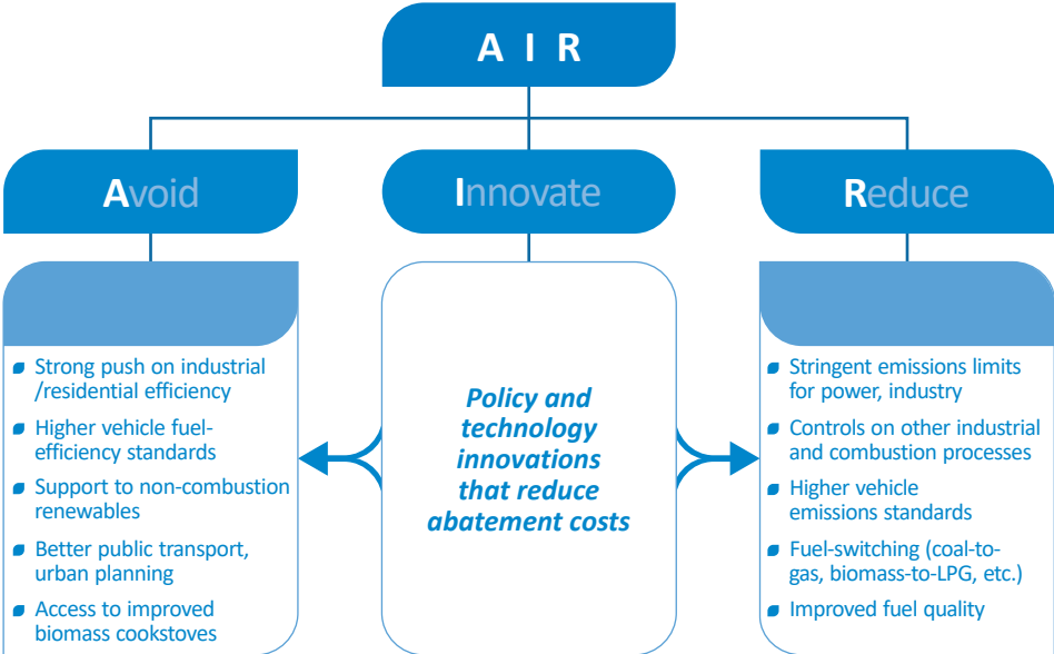
Figure 3.2 ▶ An “A-I-R” typology of energy sector actions on air pollution included in the Clean Air Scenario
