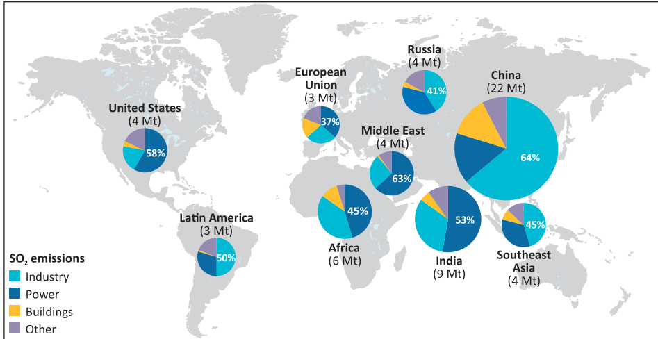
Figure 1.4 ▶ Energy-related SO 2 emissions by region and sector, 2015
