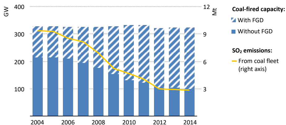
Figure 4.2 ▶ Coal power capacity equipped with flue-gas desulfurisation and related SO 2 emissions in the United States
