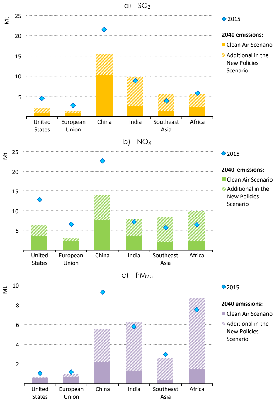
Figure 2.7 ▶ Air pollutant emissions savings by type and selected regions in the Clean Air Scenario relative to the New Policies Scenario
