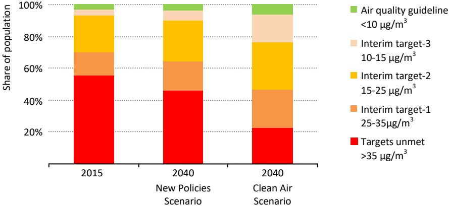
Figure 7.9 ▶ Population in China exposed to different PM 2.5 concentration levels according to WHO targets, by scenario
