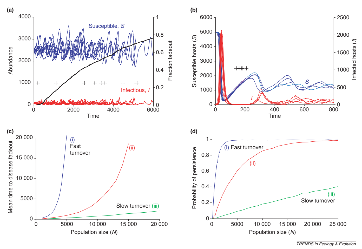
Figure 2. Endemic and epidemic fadeout and the absence of abrupt persistence thresholds illustrated using a stochastic simulation of disease spread. Results demonstrate that both types of fadeout depend strongly on demographic rates and vary gradually with N rather than showing abrupt thresholds. The simulation model tracks the numbers of S , I and R individuals and extends the model used in Figure 1 to include population recruitment and death. For all simulations, R_0=4 and recovery rate \gamma=0.1 ; (a) Endemic fadeout: ten stochastic simulations of endemic disease dynamics, begun from endemic equilibrium conditions (see Box 1). + signs indicate instances of endemic fadeout when I fluctuated to zero. The black line shows the cumulative fraction of runs with disease fadeout, out of 1000 stochastic simulations. The ratio of the mean host lifespan to mean infectious period, \alpha , equals 101. (b) Epidemic fadeout: 10 stochastic simulations of epidemic disease dynamics, begun with S=4999 , I=1 , R=0 . + signs indicate instances of epidemic fadeout during the trough in I following the first epidemic peak. \alpha equals 34.3. (c) Average time to endemic fadeout (out of 1000 runs started at the endemic equilibrium) as a function of population size and the relative rate of demographic turnover. For curves (i), (ii) and (iii), \alpha equals 51, 101 and 201, respectively. (d) Probability of persisting through the first inter-epidemic trough as a function of population size and the relative rate of demographic turnover, estimated from the fraction of 10 000 runs that persisted (starting with S=N^*-1 , I=1 , and R=0 , conditional on successful invasion of the disease). For curves (i), (ii) and (iii), \alpha equals 21, 34.3 and 51, respectively; when \alpha=101 , no runs persisted through the first trough. For full details, please see Online Supplementary Information.
