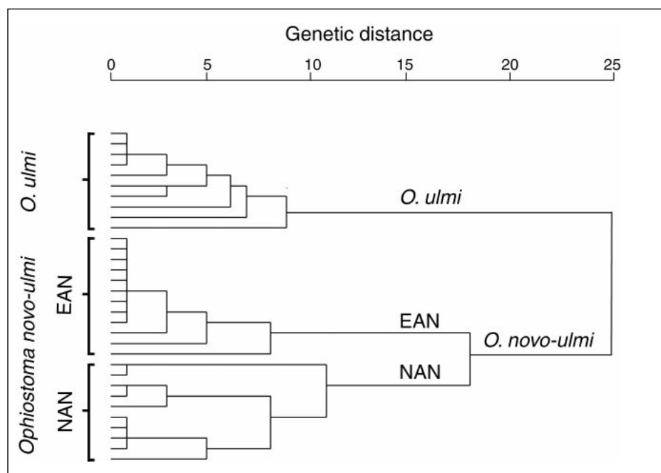
Figure 3. The phylogenetic relationship between isolates of Ophiostoma ulmi and the EAN and NAN forms of O. novo-ulmi , based on their molecular fingerprints (RFLPs of mitochondrial DNA; in this case, a PvuII digest). Adapted from Bates et al. (1993).
