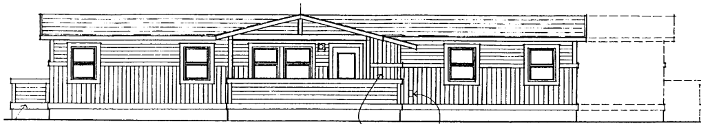
ELEVATION @ Entrance (Including site-constructed deck)
