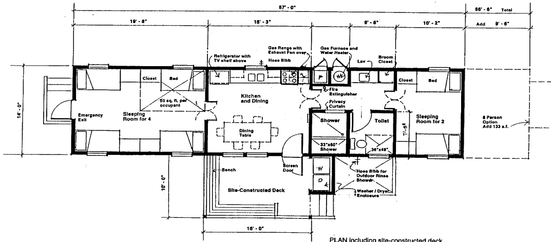
PLAN Including site-constructed deck
