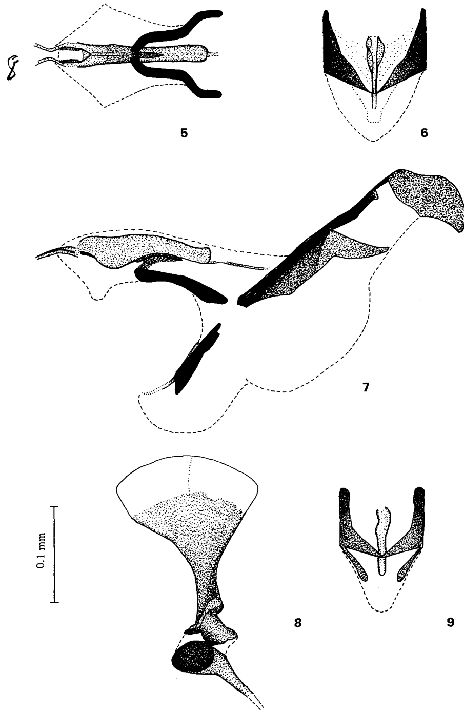
Fig. 5-8. Phytomyza petiolaris n. sp., holotype ♂ : 5, distal section of aedeagus in ventral view; 6, medial lobe of aedeagus in \pm posteroventral view; 7, aedeagus in lateral view; 8, ejaculatory apodeme. Fig. 9. Phytomyza mertensiae Sehgal (holotype ♂), medial lobe of aedeagus in \pm posteroventral view.
