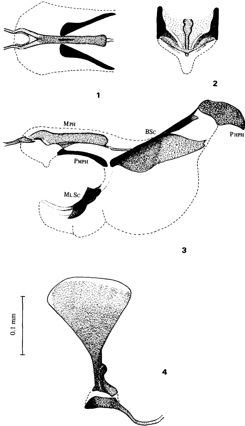
Fig. 1-4. Phytomyza ovalis n. sp., holotype ♂ : 1, distal section of aedeagus in ventral view; 2, medial lobe of aedeagus in \pm posteroventral view; 3, aedeagus in lateral view (BSc basal sclerites, MLSc sclerites of medial lobe, MPH mesophallus, PMPH paramesophallus, PPHP phallosophore); 4, ejaculatory apodeme.
