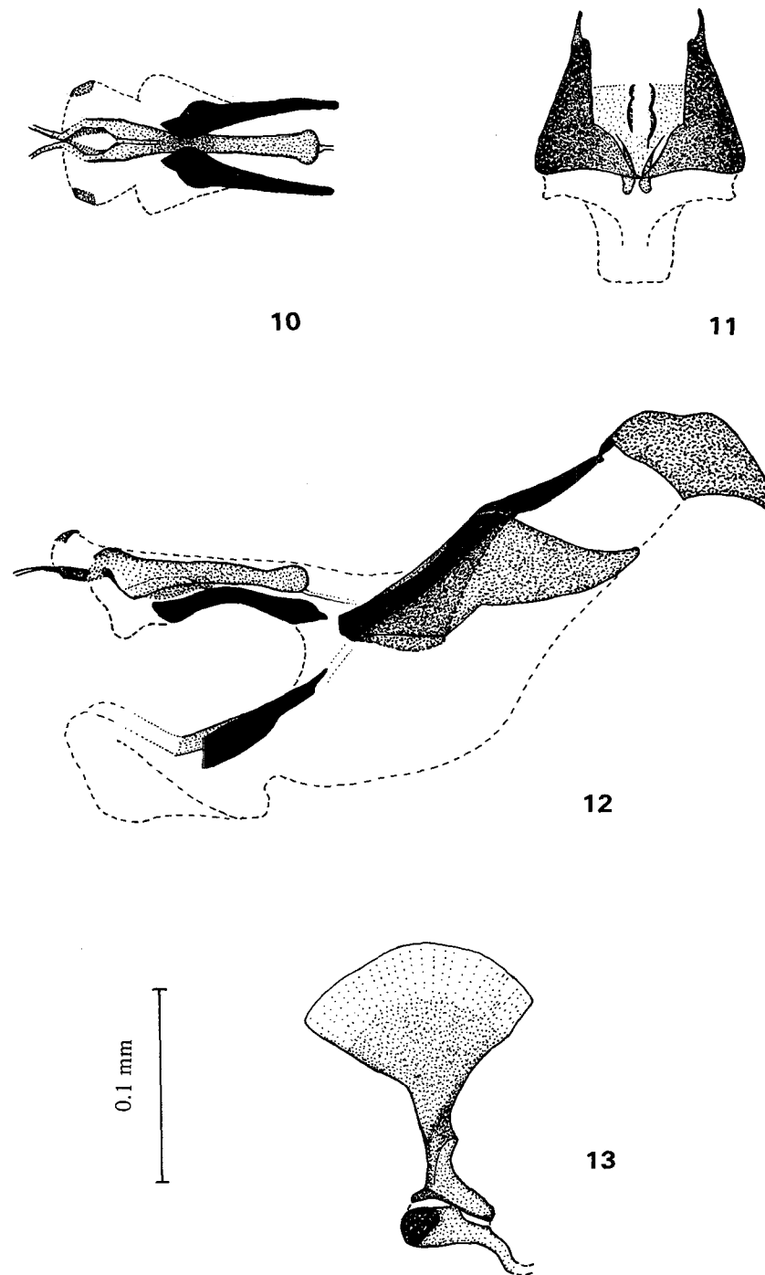
Fig. 10-13. Phytomyza beringiana n. sp., holotype ♂ : 10, distal section of aedeagus in ventral view; 11, medial lobe of aedeagus in \pm posteroventral view; 12, aedeagus in lateral view; 13, ejaculatory apodeme.
