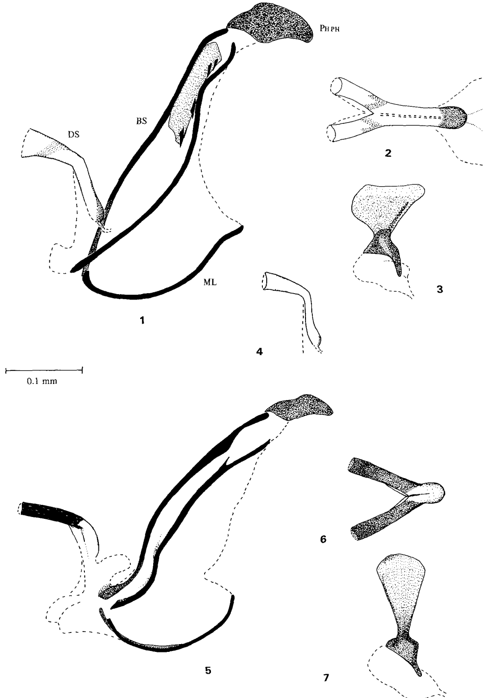
Fig. 1-3. Phytomyza asterophaga Spencer (♂): 1, aedeagus in left lateral view (BS basal section of aedeagus, DS distal section of aedeagus, ML medial lobe, PHPH phallosophore); 2, distal section of aedeagus in \pm anteroventral view; 3, ejaculatory bulb and apodeme. Fig. 4. Phytomyza ciliolati Spencer (♂), distal section of aedeagus in left lateral view. Fig. 5-7. Phytomyza despinosa n. sp., holotype ♂: 5, aedeagus in left lateral view; 6, distiphallus in dorsal view; 7, ejaculatory bulb and apodeme.
