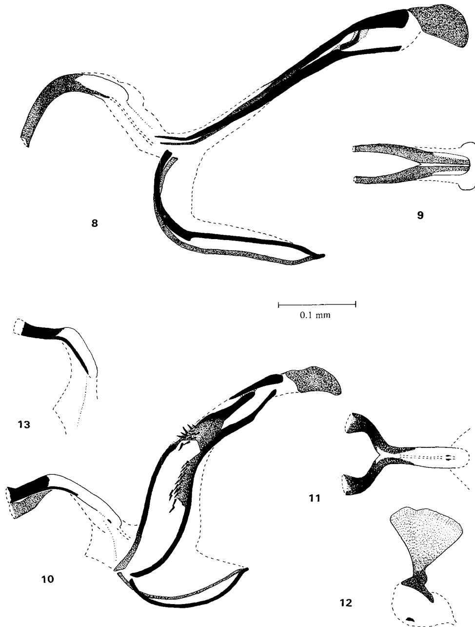
Fig. 8-9. Phytomyza solidaginivora Spencer, holotype ♂: 8, aedeagus in left lateral view; 9, distiphallus in \pm anterodorsal view. Fig. 10-12. Phytomyza phalangites n. sp., holotype ♂: 10, aedeagus in left lateral view; 11, distal section of aedeagus in ventral view; 12, ejaculatory bulb and apodeme. Fig. 13. Phytomyza astotinensis n. sp. (holotype ♂), distal section of aedeagus in left lateral view.
