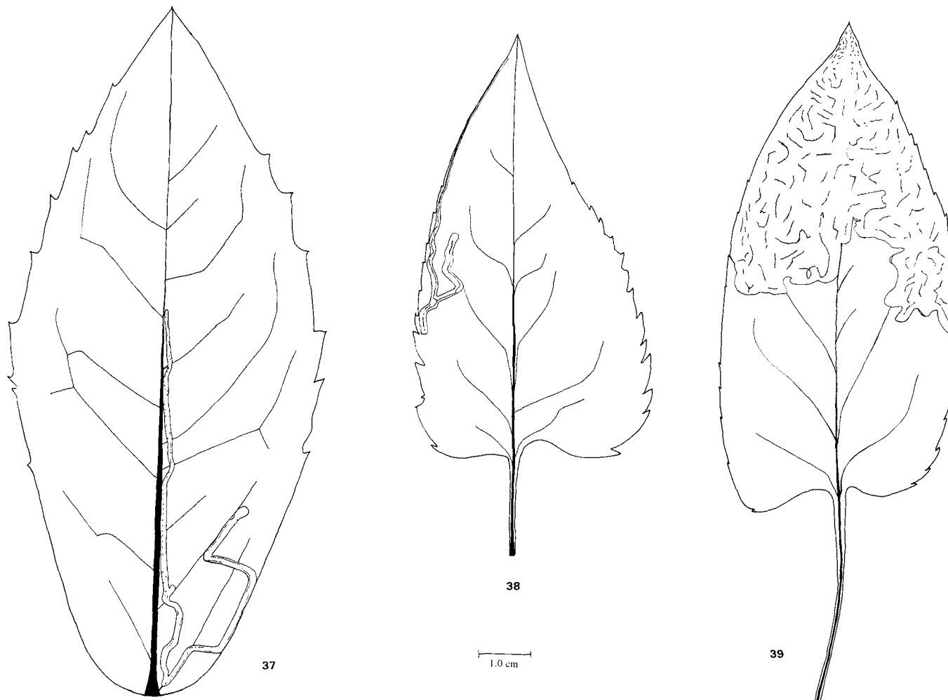
Fig. 37. Leaf of Aster conspicuus Lindl. with mine of Phytomyza asterophaga Spencer. Fig. 38-39. Leaves of Aster ciliolatus Lindl. with mines of: 38, Phytomyza ciliolati Spencer; 39, Phytomyza phalangites n. sp. (communal mine).
