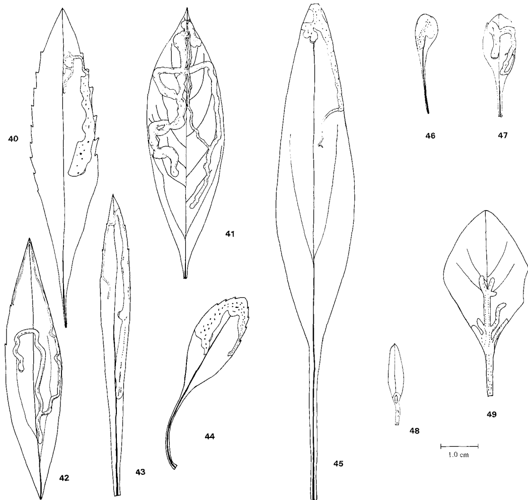
Fig. 40. Leaf of Aster sibiricus L. with mine of Phytomyza despinosa n. sp. Fig. 41. Leaf of Astereae sp. (probably Aster modestus Lindl.) with mine of Phytomyza solidaginivora Spencer. Fig. 42-43. Leaves of Solidago canadensis L. with mines of: 42, Phytomyza astotinensis n. sp.; 43, Phytomyza solidaginophaga Sehgal. Fig. 44. Leaf of Solidago multiradiata Ait. with mine of Phytomyza scopulina n. sp. Fig. 45. Leaf of Erigeron peregrinus (Pursh) subsp. callianthemus (Greene) with mine of Phytomyza peregrini n. sp. Fig. 46. Leaf of Erigeron caespitosus Nutt. with mine of Phytomyza ovimontis n. sp. Fig. 47. Leaf of Erigeron glabellus glabellus Nutt. with mine of Phytomyza erigerophila Hering. Fig. 48. Leaf of Erigeron eriocephalus J. Vahl with terminal part of mine of Chromatomyia erigerontophaga (Spencer). Fig. 49. Leaf of Erigeron philadelphicus L. with mine of Chromatomyia thermarum n. sp.
