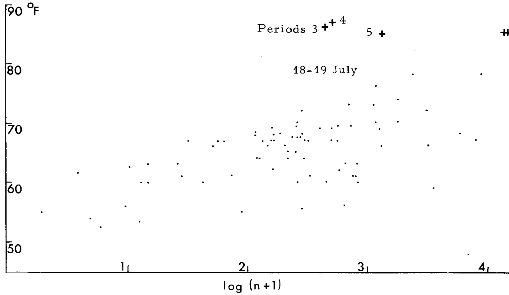
Figure 9 - Temperature against numbers of Trichoptera (as \log(n + 1) ) taken at an ultra-violet light trap at Ile Ste. Hélène, Montreal, summer 1964. Each 1 hour inter-peak period for all catch nights plotted separately.
