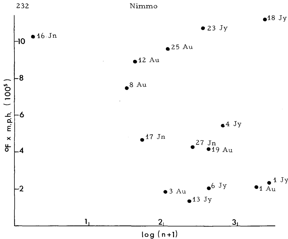
Figure 8 - Meantemperature X mean wind speed against mean log (n + 1) of inter-peak catch of Trichoptera.
